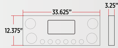
▲ RED STOP, TURN & TAIL TO PURPLE AUXILIARY TU-9001L5 Clear Lens
