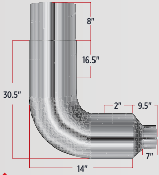
▲ 10" REDUCED TO 5" DIAMETER TEL-105
