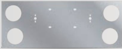
4 x 4" HOLES TU-9017
