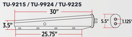
▲ PAINTED STEEL TU-9225
