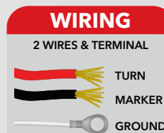
CLEAR AMBER/RED TURN & MARKER TLED-FDC
