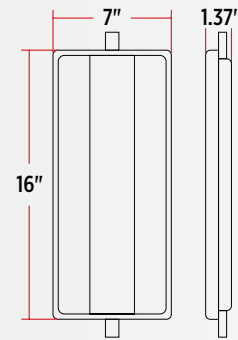
▲ HEATED WITH INCANDESCENT TM-2011
