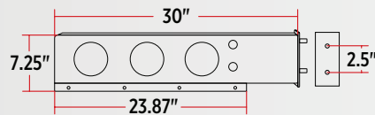
▲ RED STOP, TURN & TAIL TU-9210L1 Red Lens
