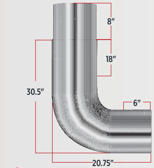
▲ 8" DIAMETER TEL-8
