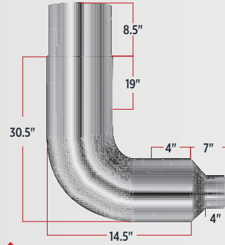
▲ 8" REDUCED TO 5" DIAMETER TEL-85
