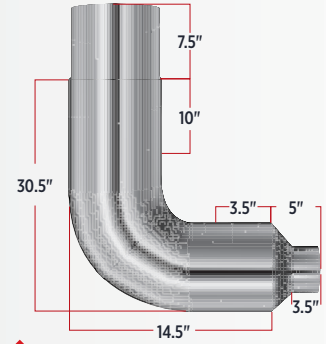
▲ 6" REDUCED TO 5" DIAMETER TEL-65
