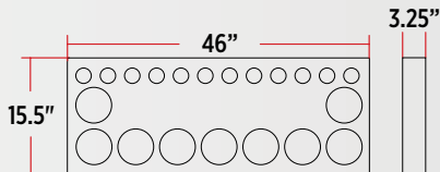
RED STOP, TURN & TAIL TU-9013LC Clear Lens
