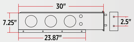
RED STOP, TURN & TAIL TO GREEN AUXILIARY TU-9210L5 Clear Lens
