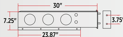
▲ RED STOP, TURN & TAIL TU-9209L1 Red Lens
