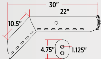
▲ PAINTED STEEL TU-9222
