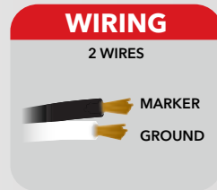
CLEAR AMBER MARKER TLED-CABC
