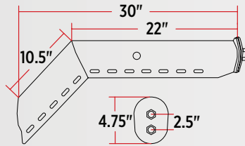
▲ PAINTED STEEL TU-9228
